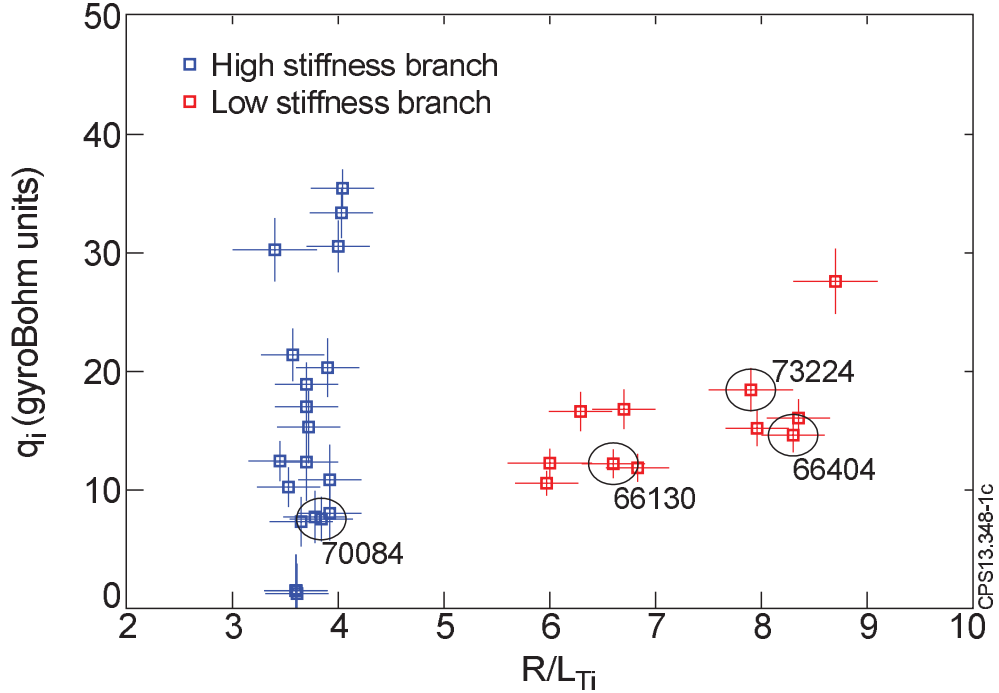
FIG. 1. Ion heat flux versus R/L_{Ti} , from JET data presented in Ref. [7] showing a separation between high and low stiffness regimes at \rho = 0.33 . The specific discharges studied in this Letter are circled.
