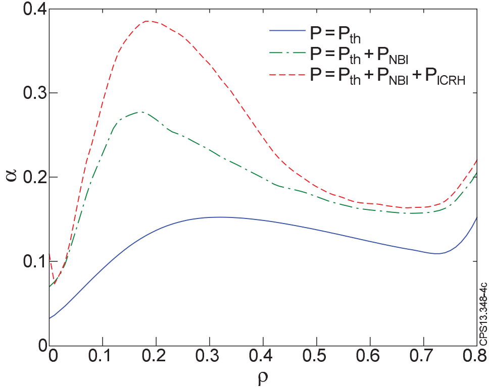
FIG. 4. The comparative influence of thermal and suprathreshold pressure components on \alpha for discharge 66404. Increased \alpha corresponds qualitatively to increased electromagnetic stabilization. The strong influence of suprathreshold pressure for \rho < 0.4 coincides with the measured low stiffness zone.
