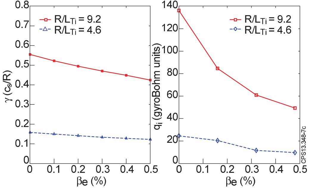
FIG. 3. Linear growth rates (a) and nonlinear ion heat fluxes (b) calculated in \beta_e and R/L_{Ti} scans based on discharge 66404 parameters. In the linear scan, k_y = 0.4 in units of 1/\rho_s . Runs included collisions, experimental geometry, two species, and assumed T_e/T_i = 1 .
