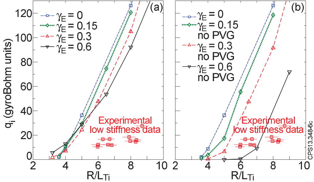
FIG. 2. Ion heat flux in nonlinear GENE R/L_{Ti} and \gamma_E scans based on discharge 70084 parameters at \rho = 0.33 ( q/\epsilon = 11.8 for circular geometry). \hat{s}/q = 0.2/1.3 throughout. Results are shown both including (a) and neglecting (b) PVG destabilization. All runs were electrostatic, collisionless, used circular geometry, and assumed T_e/T_i = 1 . The results are compared with the low stiffness data from Ref. [7].
