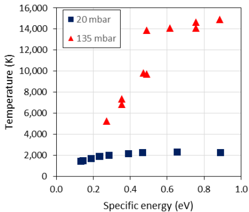
FIG. 5: Gas temperatures determined from neutral gas density measurements with Rayleigh scattering and reactor pressure readings in a scan of specific energy input. The gas flow was at 13 slm similar to the high flow conditions in Figure 3 and 4, the pressure was tuned to 20 and 135 mbar, respectively.
