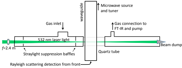
FIG. 1: Schematic of the microwave plasma source used for CO 2 dissociation. Indicated is the laser beam path that is used for Rayleigh scattering experiment.
