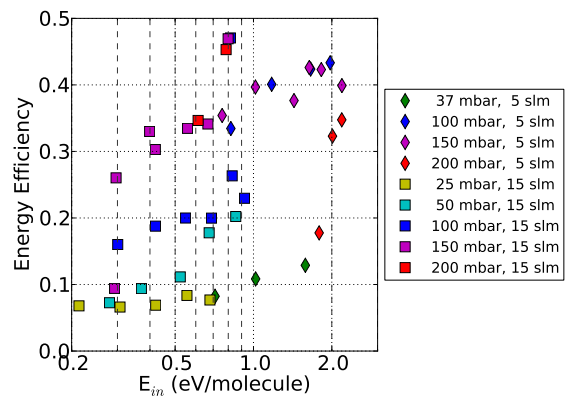
FIG. 4: Energy efficiency measured in pure microwave CO 2 plasma as a function of the specific energy input, at 5 and 15 slm gas flow rate, in scans of the reactor pressure. The underlying experimental data are identical to those of Figure 3.
