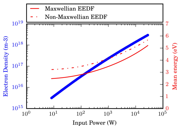
FIG. 6: Electron density (left axis) and mean energy (right axis) calculated as a function of input power for a CO 2 microwave discharge. Compared are solutions of the balance equations assuming a Maxwellian EEDF and solutions which involved detailed Bolsig + calculations of the EEDF. The non-Maxwellian nature leads to increased mean electron energies. Dissociative recombination becomes more important as density increases, which causes the increase in mean electron energy with input power. Assumed was a neutral gas density of 10^{23} \text{ m}^{-3} , which is similar to measured values.
