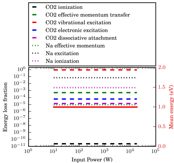
FIG. 10: The effect of 0.01% sodium added to a CO 2 microwave discharge on the relative energy loss fractions for the main processes at play. It shows that vibrational excitation has become the dominant energy loss channel for the electrons, which does not change within the conditions as investigated in the present work.
