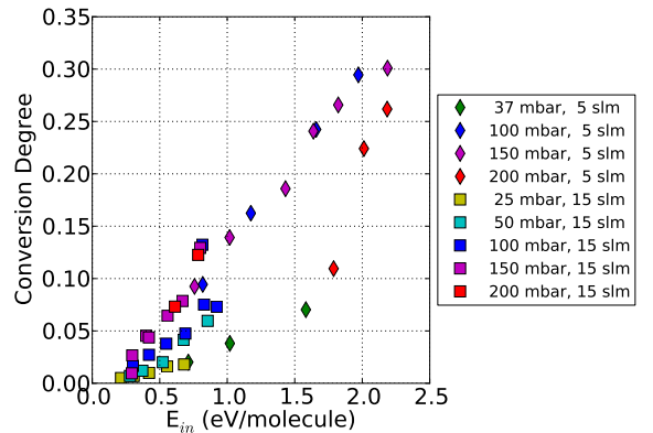
FIG. 3: Conversion degree measured in pure microwave CO 2 plasma as a function of the specific energy input, at 5 and 15 slm gas flow rate, in scans of the reactor pressure.
