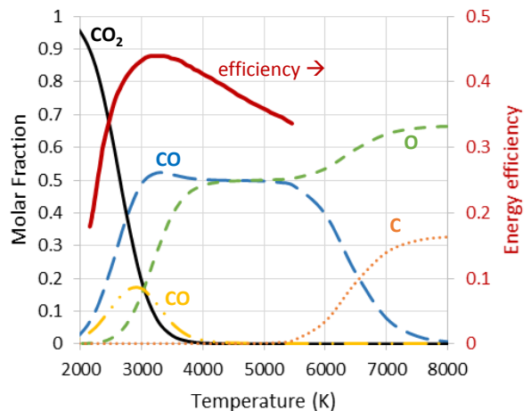
FIG. 8: Chemical Equilibrium calculated molar fraction of the products of \text{CO}_2 dissociation at a fixed pressure of 100 mbar. Calculated energy efficiencies assuming instantaneous quenching after Polak et al. are plotted on the right axis.
