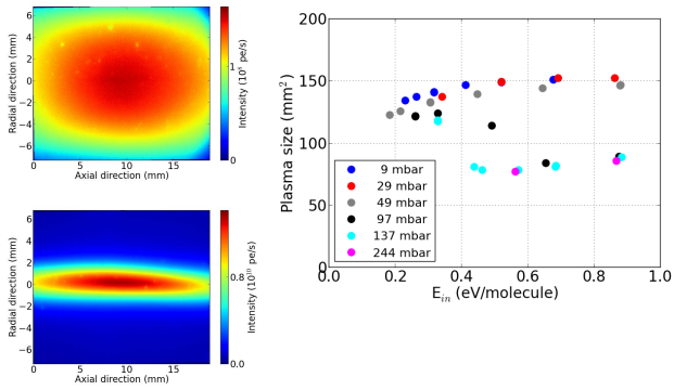
FIG. 2: Spontaneous light emission from the plasma inside the waveguide for (left top) 10 mbar (650 W, 13 slm) and (left bottom) 250 mbar (550 W, 13 slm), illustrating the two modes of operation: diffuse and contracted.[1] It is noted that vignetting at the sides of the images was not corrected for. The plot on the right shows the plasma cross sectional area determined from such emission images in dependence of pressure and specific energy. Plasma cross sectional areas of 120-150 mm 2 and 80 mm 2 corresponds to diffuse and contracted operation, respectively.
