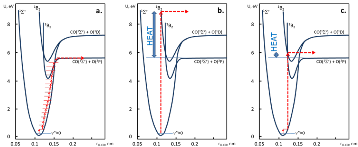
FIG. 11: Potential energy diagrams (as a function of one O-CO bond length) that illustrate the molecular physics behind three variants of \text{CO}_2 dissociation. Diagram (a) represents stepwise vibrational excitation that, after term crossing, causes ideally efficient dissociation. Contrary is dissociative excitation in diagram (b), which involves a significant amount of heat to be released. A mix of these two cases is shown in diagram (c): vibrationally activated dissociative excitation, which is shown here as highly efficient as well.
