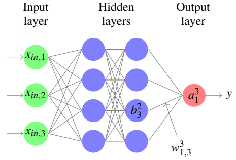
FIG. 8. A schematic representation of a two-hidden-layer feed-forward neural network. w_{jk}^l is the weight of the connection from the k^{\text{th}} neuron in the (l-1)^{\text{th}} layer to the j^{\text{th}} neuron in the l^{\text{th}} layer. Then, b_j^l is the bias of the j^{\text{th}} neuron in the l^{\text{th}} layer. The final network output is the activation of the j^{\text{th}} neuron in the l^{\text{th}} layer.
