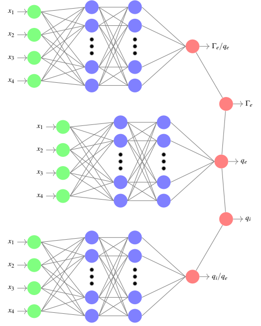
FIG. 9. Schematic overview of the \Gamma_e and q_e predicted by a combined leading flux and ratio-predicting neural network for TEM fluxes. Three separate FFNNs, one predicting the leading flux q_e and two ratio-predicting network predicting \Gamma_e/q_e and q_i/q_e are combined to a network ensemble that predicts \Gamma_e , q_e , and q_i .
