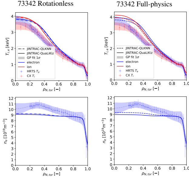
FIG. 3. The final kinetic profiles of the JINTRAC-QuaLiKiz (solid) and JINTRAC-QLKNN (dash-dot) simulations of JET shot #73342. Shown are the final temperatures for the ions (top, red) and electrons (top, blue) as well as the final electron density (bottom, blue). Both cases were run with interpretive impurities without rotation (left) and with rotation (right). The QLKNN predictions lie close to the QuaLiKiz ones, in the order of 4% at maximum, which show the generality of applying QLKNN as quicker surrogate for the full QuaLiKiz model. We do note the underprediction of the density profile by QuaLiKiz. This is a known issue at high collisionality, which is currently under investigation by the QuaLiKiz team, and a revision of the collisionality model will be included in future releases.
