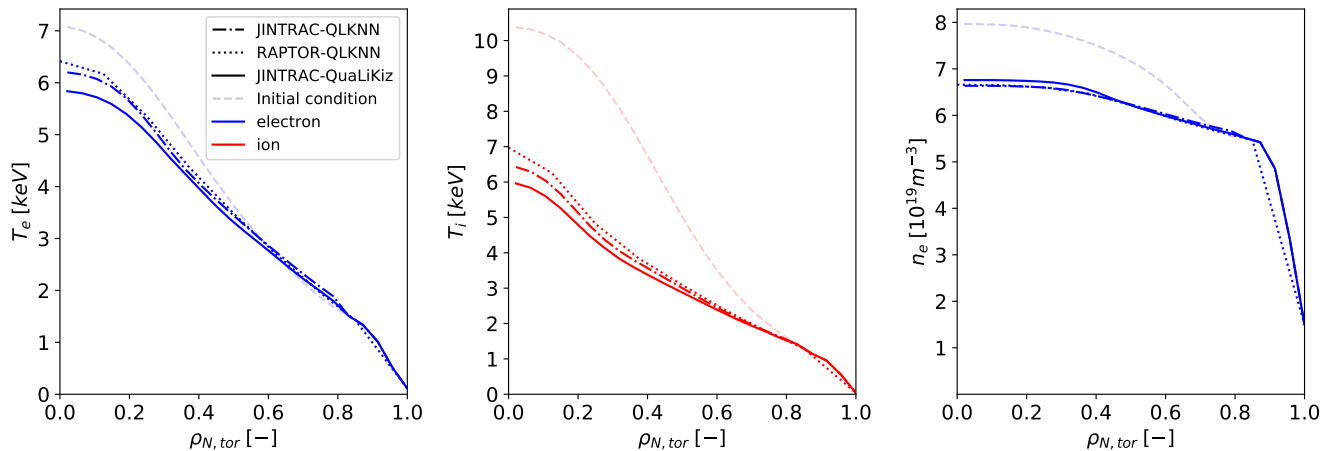
FIG. 1. The final kinetic profiles of the JINTRAC-QuaLiKiz (solid) and JINTRAC-QLKNN (dash-dot) and RAPTOR-QLKNN(dot) simulations of JET shot #92436. Shown are the final temperatures for the electrons (left, blue) and ions (middle, red) as well as the final electron density (right, blue). We also show the initial condition from GP regression in dashes. The simulations were done with low physics fidelity to aid the benchmark, most notably without rotation and with a pure plasma. The agreement between the three simulations is remarkable, within 5.5% of each other. The QLKNN simulations were three orders of magnitude faster than the JINTRAC-QuaLiKiz one. Remaining small differences between JINTRAC and RAPTOR are likely caused by the different numerical schemes, and are currently under investigation.
