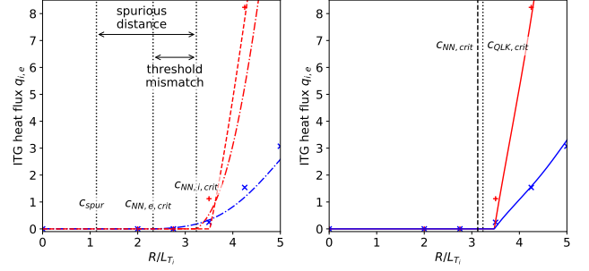
FIG. 11. Predictions of the ITG driven heat flux for the ions (red) and electrons (blue). We show three types of networks trained using a standard RMS error on both the stable and unstable points (dash-dot, left) and only on the unstable points (dashed, left). These networks show clear mismatch between transport channels and QuaLiKiz prediction, as well as a small but finite prediction of fluxes in the stable region. The physics-based neural network (right) have no mismatch between transport channels, a sharper threshold closer to the QuaLiKiz prediction, as well as no prediction of flux in the stable region.
