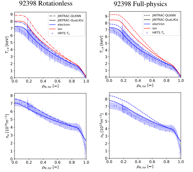
FIG. 4. The final kinetic profiles of the JINTRAC-QuaLiKiz (solid) and JINTRAC-QLKNN (dash-dot) simulations of JET shot #92398. Shown are the final temperatures for the ions (top, red) and electrons (top, blue) as well as the final electron density (bottom, blue). Both cases were run with interpretive impurities without rotation (left) and with rotation (right). Here the disagreement between QuaLiKiz and QLKNN is larger than previous cases, but still within 13%. Future improvements to the QLKNN model are expected to lower these differences, but this result shows that even in this state the QLKNN model can be used for quick exploratory studies.
