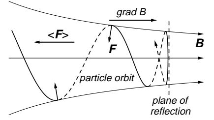
Figure 7: Reflected particle orbit in a magnetic mirror.
