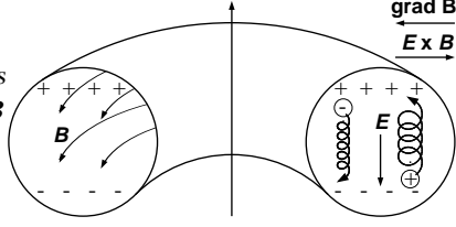
Figure 9: Vertical drifts and associated \mathbf{E} \times \mathbf{B} drift in a toroidal field.
